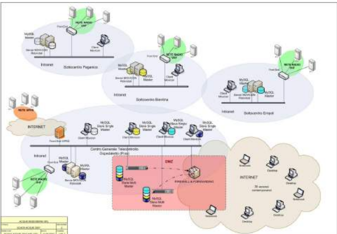
The Acque Spa remote control system architecture
