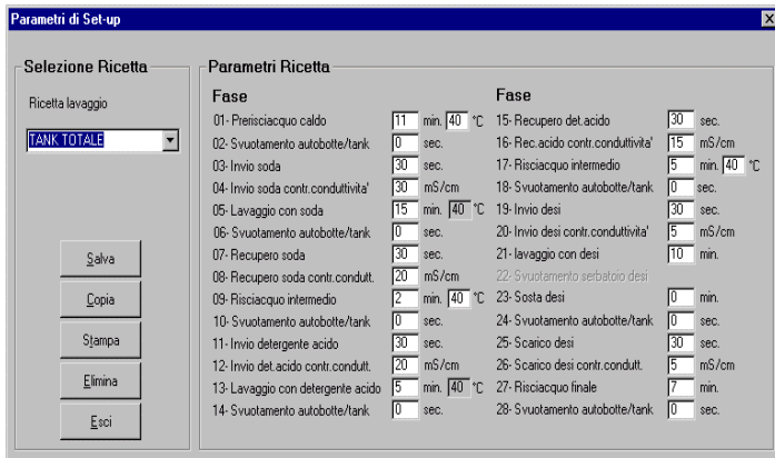
An example of the CIP system's wash parameter settings. Solutions are provided in the form of recipes to allow maximum management flexibility.
