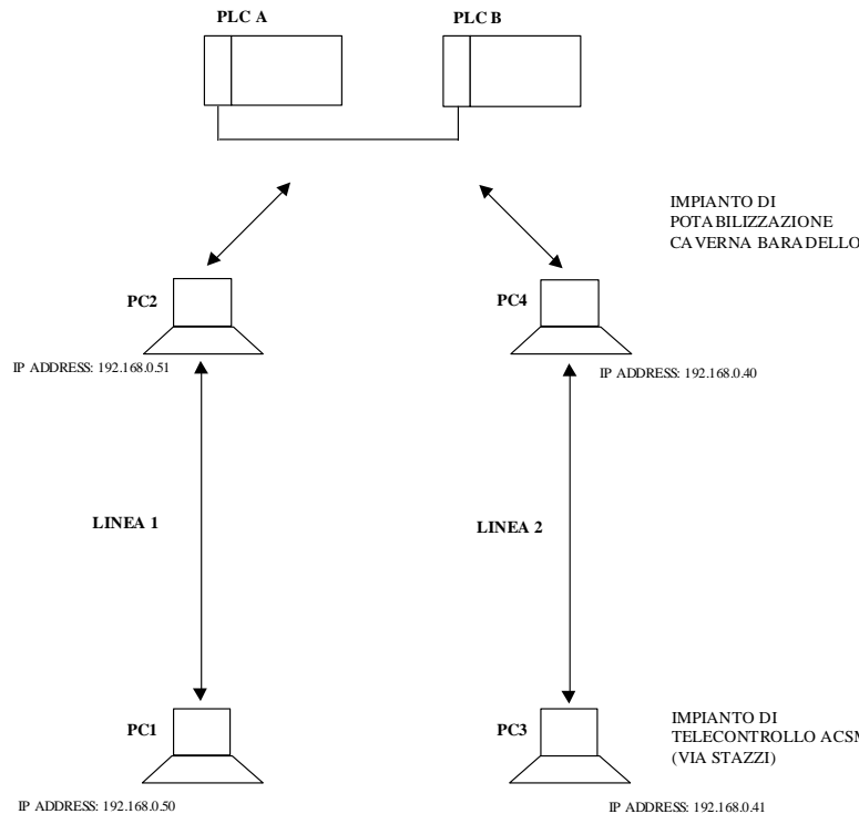
Water Purifying plant telecontrol system architecture.
